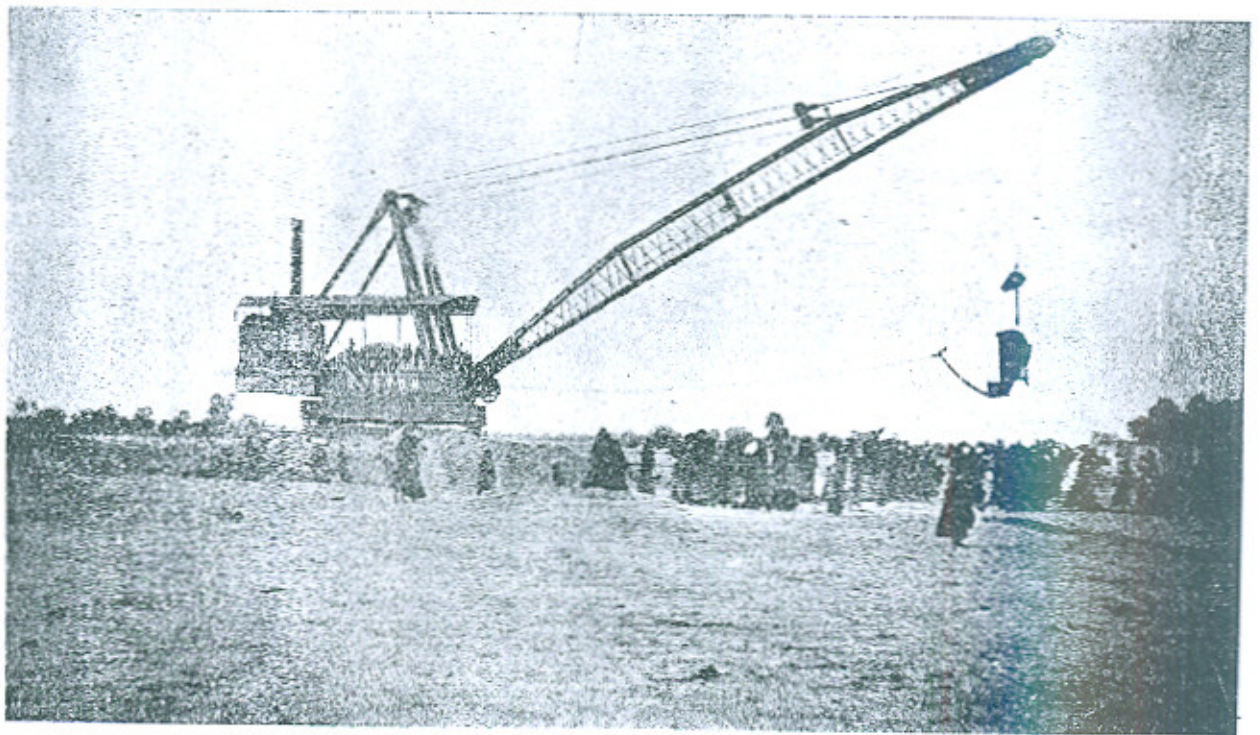
Fig. 4. A 300 TON DRAGLINE EQUIPPED WITH 8 CUB. YD. BUCKET AND 120' 0" BOOM.
